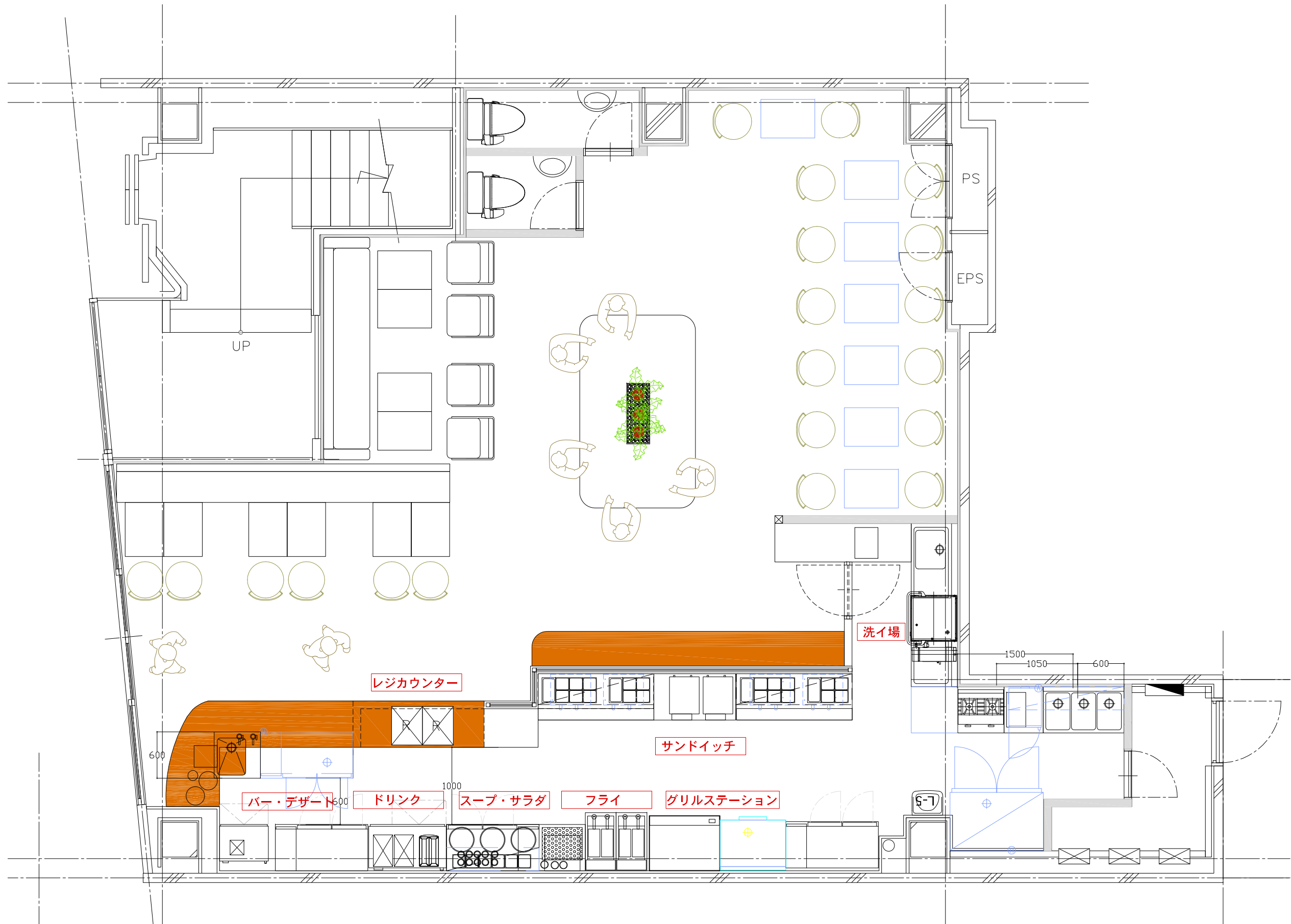
Design by Iwamoto LDKS LLC Hamburger Shop P-Type Kitchen Scale A3 = 1/50
